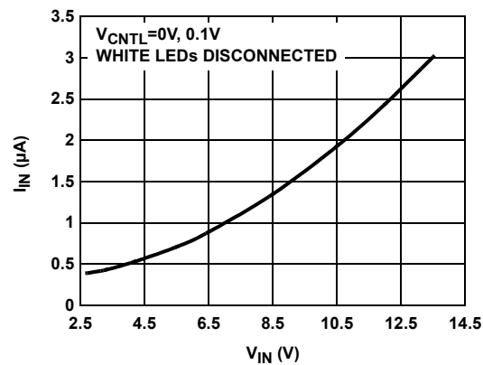
FIGURE 2. QUIESCENT CURRENT
