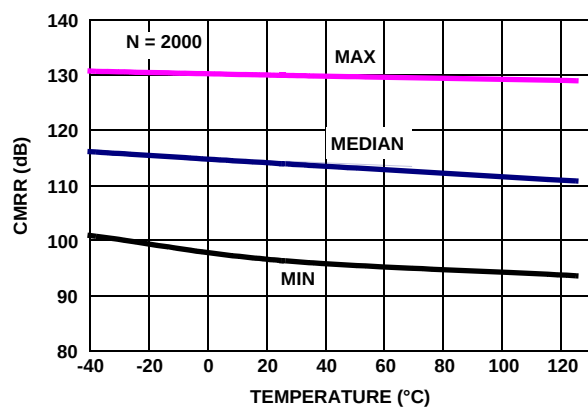
FIGURE 25. EL8170 CMRR vs TEMPERATURE, V_{CM} = +2.5V TO -2.5V , V_+ , V_- = \pm 2.5V
