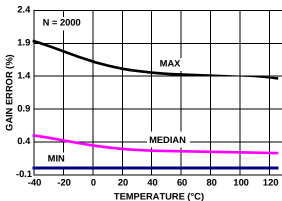
FIGURE 29. EL8170 %GAIN ERROR vs TEMPERATURE, R_L = 100k
