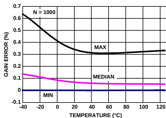
FIGURE 30. EL8173 %GAIN ERROR vs TEMPERATURE, R_L = 100k
