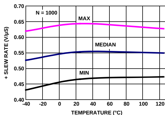
FIGURE 36. EL8173 + SLEW RATE vs TEMPERATURE, INPUT \pm 0.015V @ GAIN + 100
