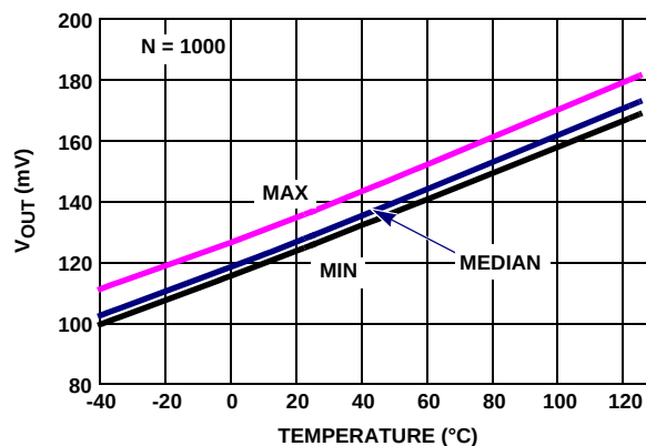
FIGURE 34. EL8173 V_{OUT} LOW vs TEMPERATURE, R_L = 1k , V_+ , V_- = \pm 2.5V
