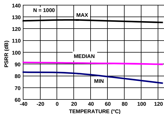
FIGURE 28. EL8173 PSRR vs TEMPERATURE, V_+ , V_- = \pm 1.2V TO \pm 2.5V
