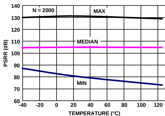
FIGURE 27. EL8170 PSRR vs TEMPERATURE, V_+ , V_- = \pm 1.2V TO \pm 2.5V
