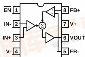
EL8170, EL8173 (8 LD SOIC) TOP VIEW
