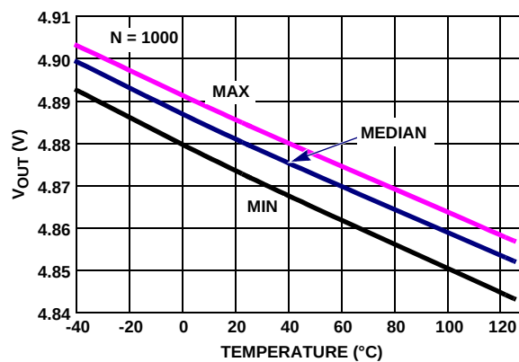
FIGURE 32. EL8173 V_{OUT} HIGH vs TEMPERATURE, R_L = 1k , V_+ , V_- = \pm 2.5V
