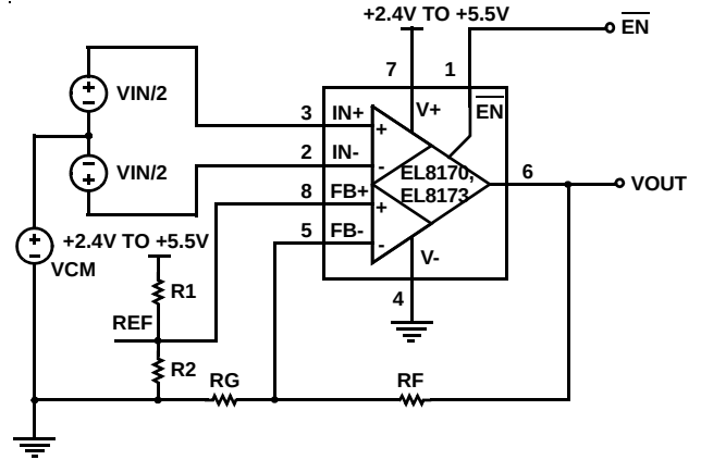
FIGURE 40. GAIN SETTING AND REFERENCE CONNECTION
