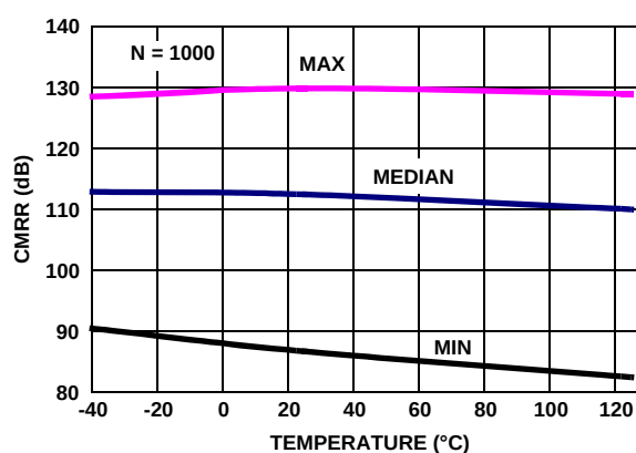
FIGURE 26. EL8173 CMRR vs TEMPERATURE, V_{CM} = +2.5V TO -2.5V , V_+ , V_- = \pm 2.5V
