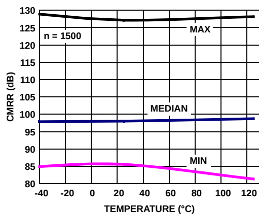
FIGURE 25. CMRR vs TEMPERATURE, V_S = \pm 2.5V , R_L = 1k
