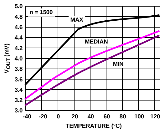
FIGURE 30. V_{OUT} LOW vs TEMPERATURE, V_S = \pm 2.5V , R_L = 100k
