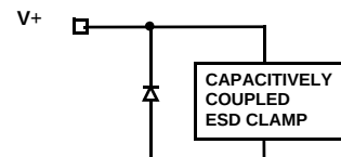
CIRCUIT 4
