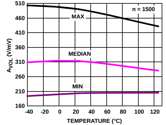
FIGURE 24. A_{VOL} vs TEMPERATURE, R_L = 100k , V_O = \pm 2V @ V_S = \pm 2.5V
