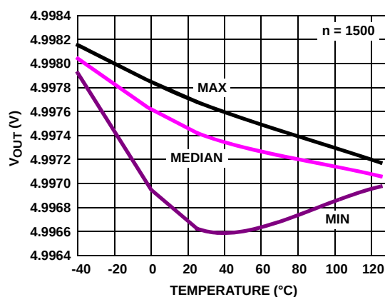
FIGURE 28. V_{OUT} HIGH vs TEMPERATURE, V_S = \pm 2.5V , R_L = 100k
