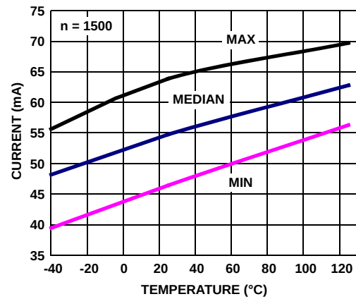
FIGURE 14. SOT-23/SO-8 ENABLED SUPPLY CURRENT vs TEMPERATURE, V_S = \pm 2.5V
