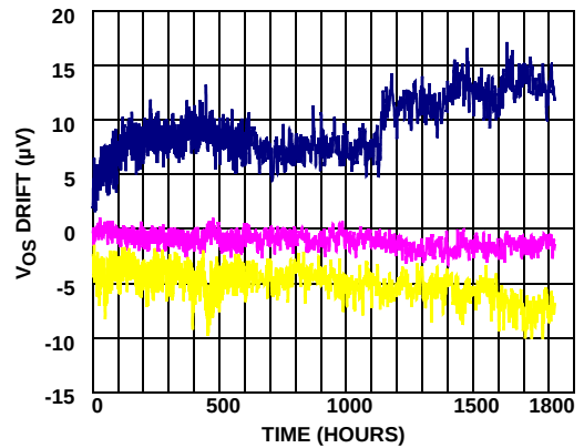
FIGURE 12. VOS DRIFT (SOT-23 PACKAGE) vs TIME
