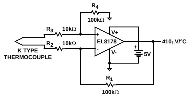
FIGURE 33. THERMOCOUPLE AMPLIFIER
