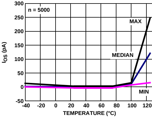
FIGURE 23. I_{OS} vs TEMPERATURE, V_S = \pm 2.5V
