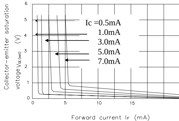
Fig. 3 Collector-emitter Saturation Voltage vs. Forward Current ( T_a=25^\circ\text{C} )
