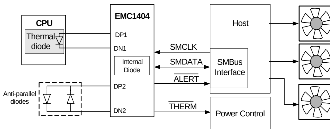
Figure 5.2 System Diagram for EMC1404
