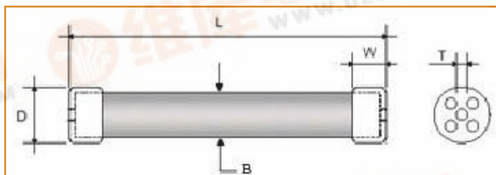
DIMENSIONS [mm]
