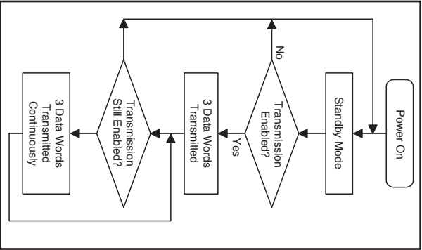
Figure 8: Encoder Flowchart
