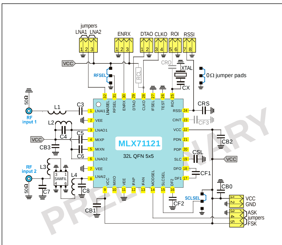
Fig. 5: Circuit schematic
