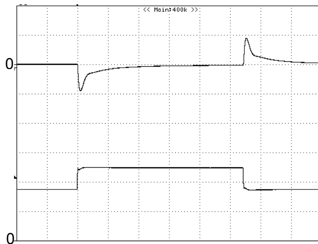
Figure 9: Output voltage response to step-change in load current (75%-50%-75% of I_o , max; di/dt = 2.5A/\mu s ). Load cap: 47\mu F , 35m\Omega ESR solid electrolytic capacitor and 1\mu F ceramic capacitor. Top Trace: V_{out} (0.2V/div, 200us/div), Bottom Trace: I_{out} (1A/div). Scope measurement should be made using a BNC cable (length shorter than 20 inches). Position the load between 51 mm to 76 mm (2 inches to 3 inches) from the module
