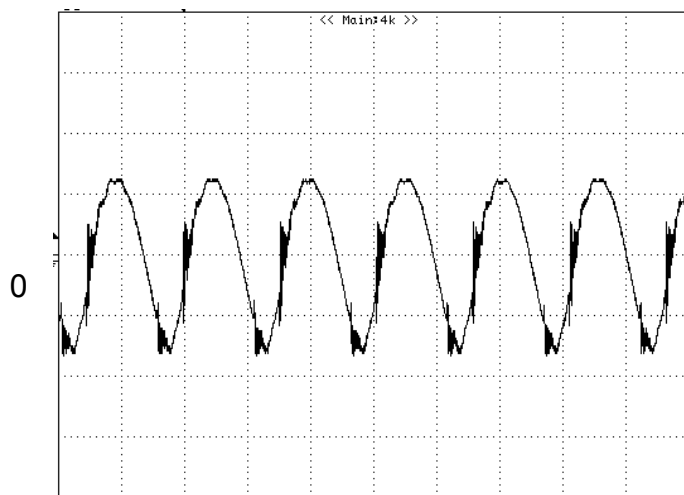
Figure 11: Input Terminal Ripple Current, i_c , at full rated output current and nominal input voltage with 12\mu H source impedance and 33\mu F electrolytic capacitor (500 mA/div, 2us/div)
