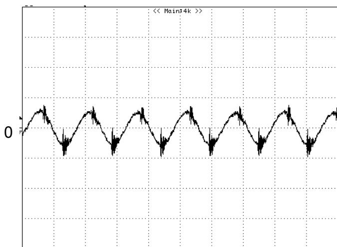
Figure 12: Input reflected ripple current, i_s , through a 12\mu\text{H} source inductor at nominal input voltage and rated load current (20 mA/div, 2 μs/div)
