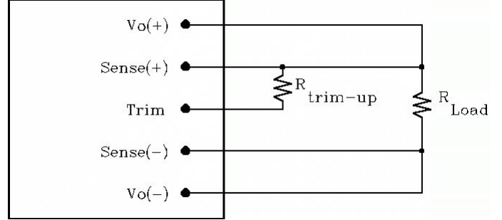
Figure 19: Circuit configuration for trim-up (increase output voltage)
