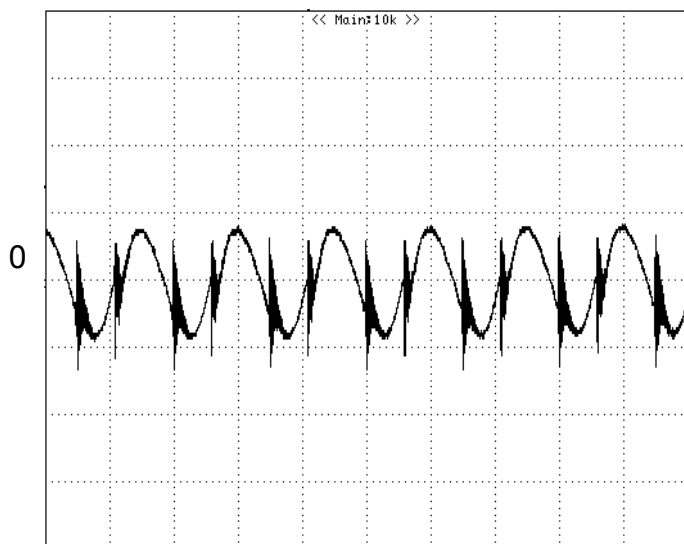
Figure 14: Output voltage ripple at nominal input voltage and rated load current ( I_o=25A )(10 mV/div, 2us/div) Load capacitance: 1 \mu F ceramic capacitor and 10 \mu F tantalum capacitor. Bandwidth: 20 MHz. Scope measurements should be made using a BNC cable (length shorter than 20 inches). Position the load between 51 mm to 76 mm (2 inches to 3 inches) from the module
