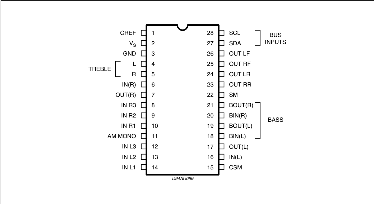
Figure 2. PIN connections
