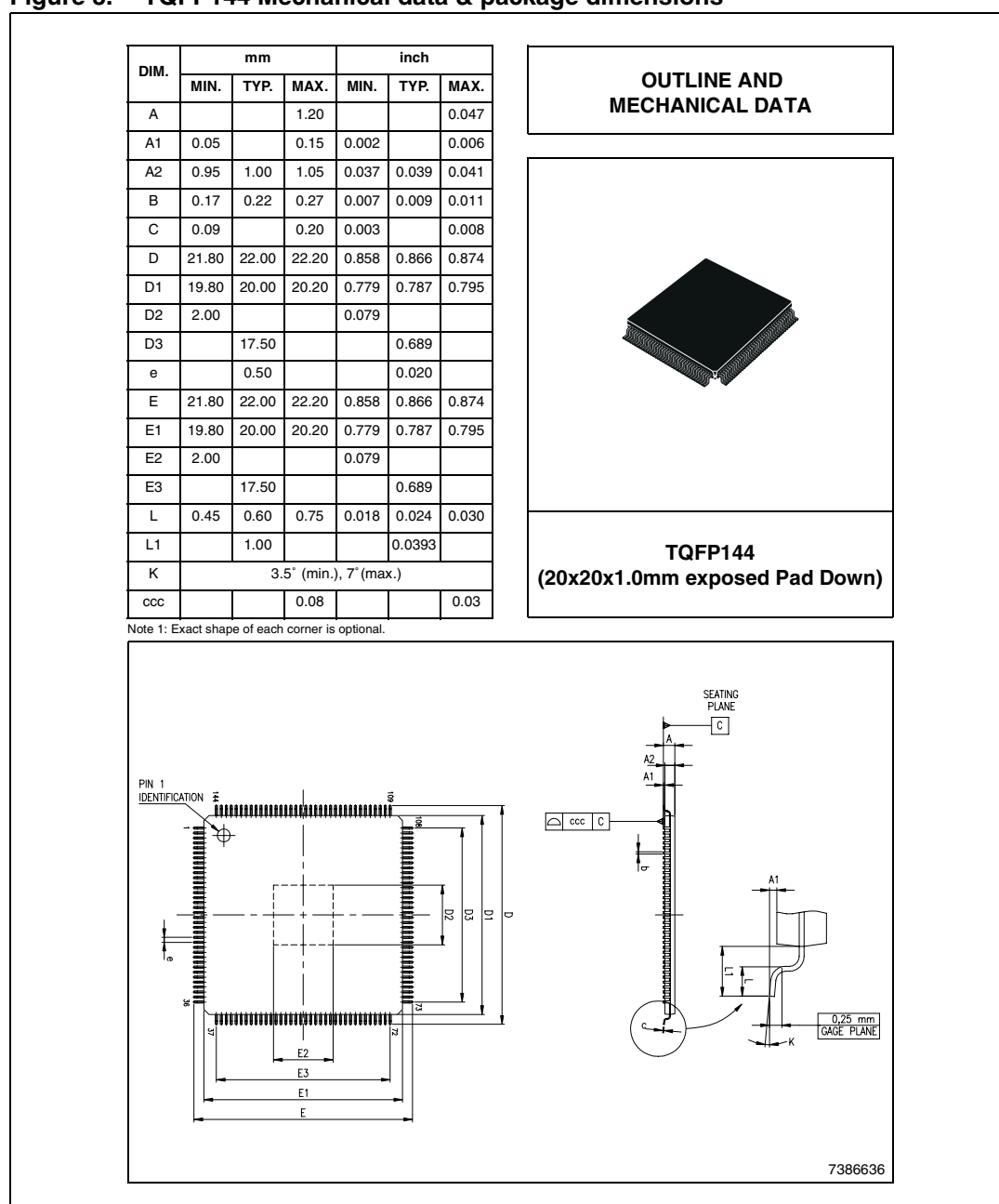
Figure 3. TQFP144 Mechanical data & package dimensions
