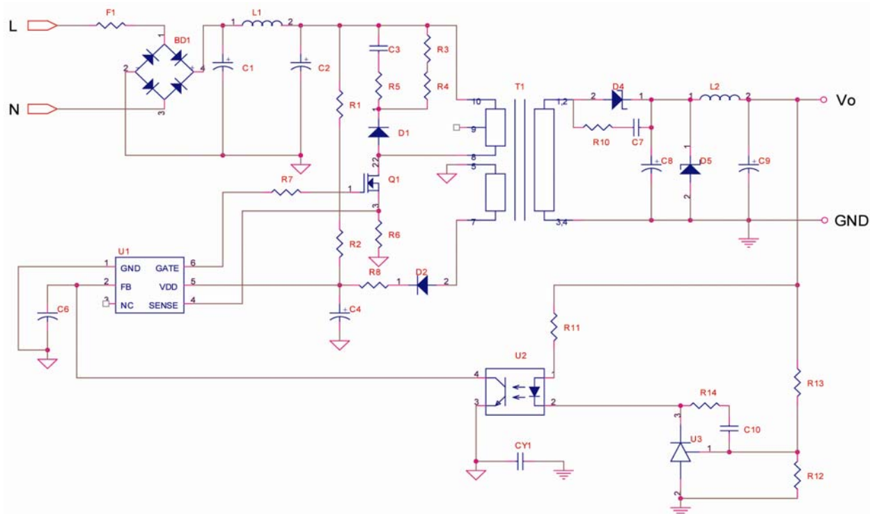
Figure 17. Reference Circuit
