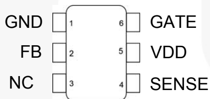
Figure 4. SSOT-6 Pin Configuration
