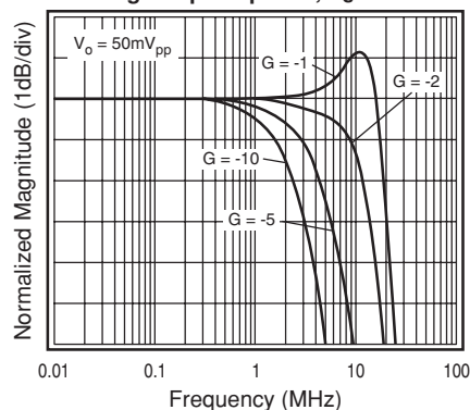
Inverting Freq. Response, V_S = 1.2\text{V}
