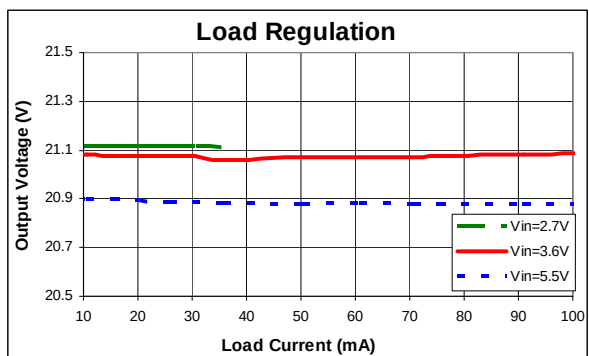
Figure 5. Load Regulation
