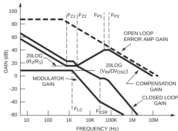
Figure 7. Asymptotic Bode Plot of Converter Gain
