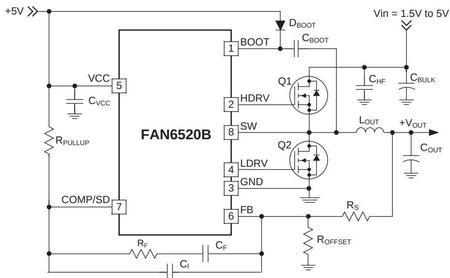
Figure 1. Typical Application
