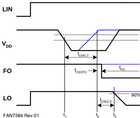
Figure 34. Waveforms for Under-Voltage Lockout
