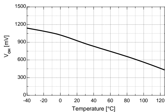
Figure 19. High-Level Output Voltage vs. Temperature
