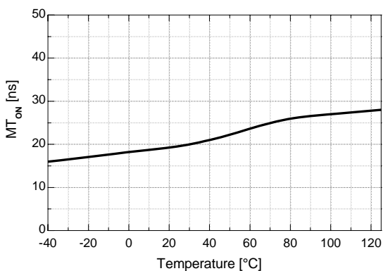
Figure 9. Turn-on Delay Matching vs. Temperature
