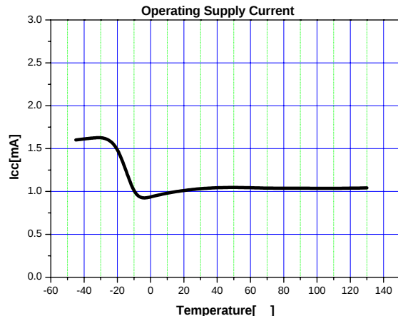
Figure 8. Operating Supply Current vs. Temp.
