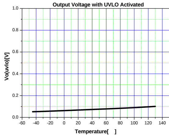
Figure 29. Output Voltage when UVLO vs. Temp.
