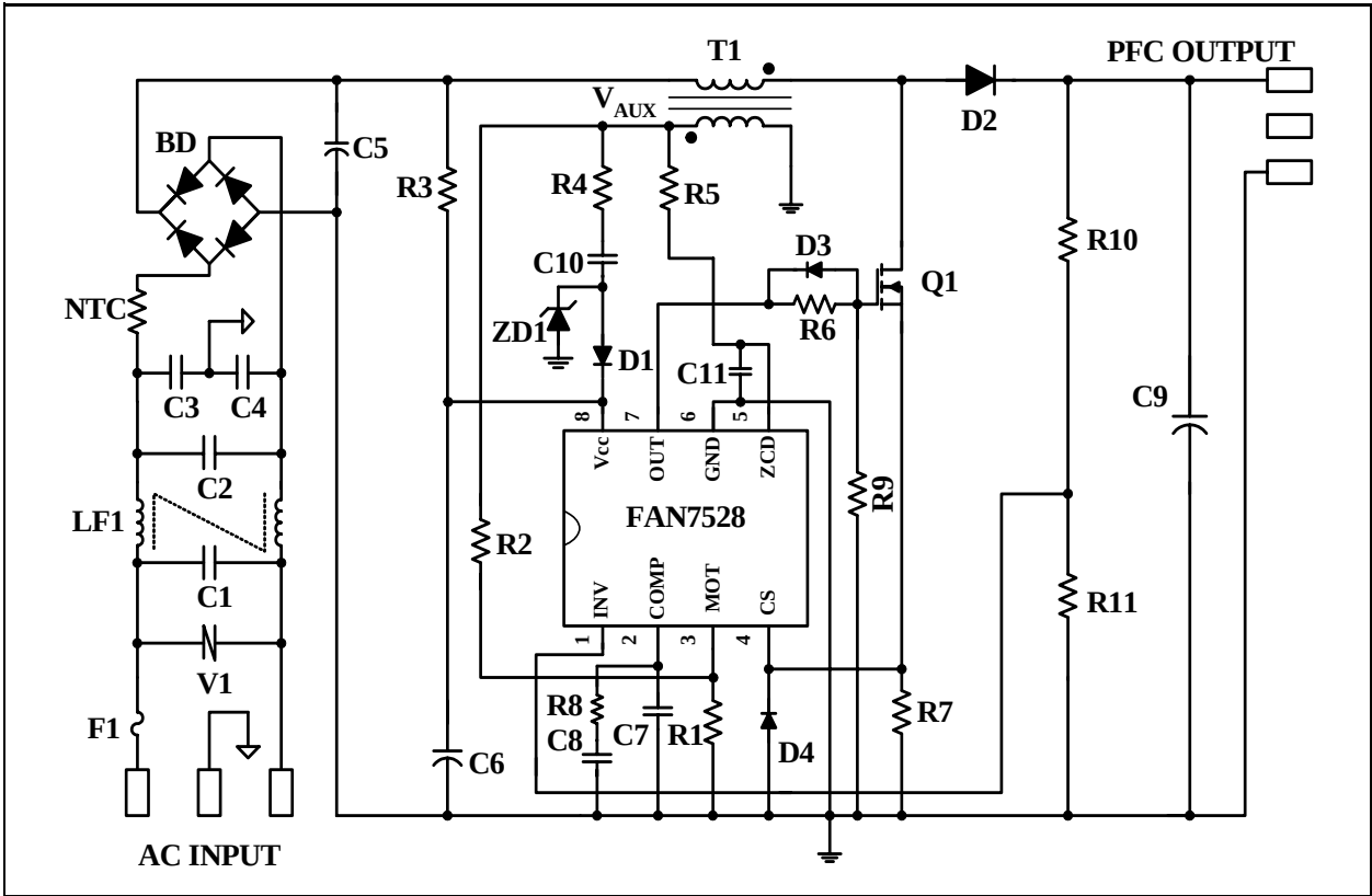
Figure 39. Schematic
