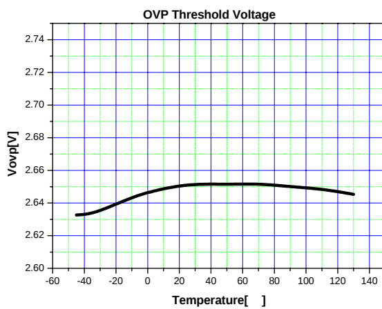
Figure 31. Over Voltage Protection vs. Temp.
