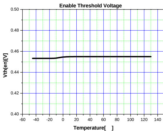
Figure 33. Enable Threshold Voltage vs. Temp.
