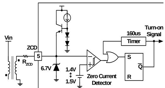
Figure 36. Zero current detector block
