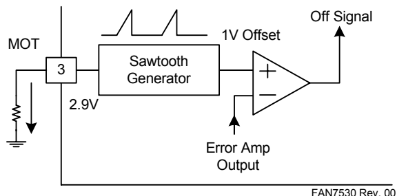
Figure 35. Sawtooth Generator Block
