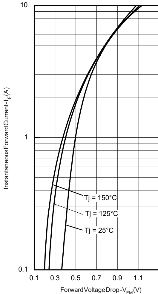
Fig. 1 - Maximum Forward Voltage Drop Characteristics (Per Leg)
