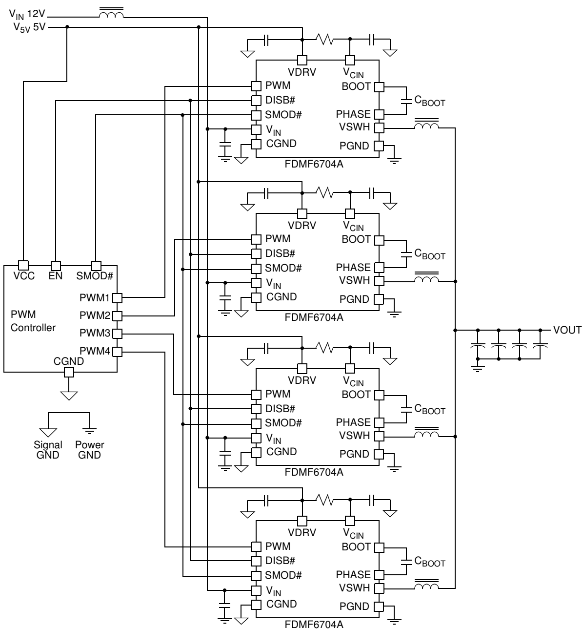
Figure 21. Typical Application
