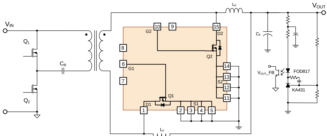
Figure 16. Application Circuit of Asymmetrical HB Converter with FD6M033N06
