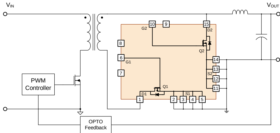
Figure 15. Application Circuit of Forward Converter with FD6M033N06
