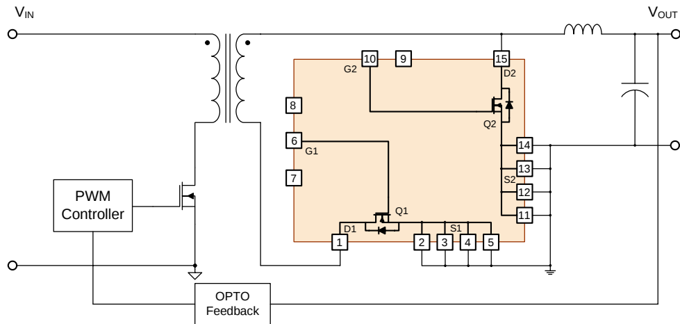
Figure 15. Application Circuit of Forward Converter with FD6M043N08
