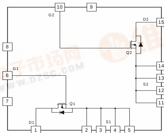
Figure 1. FD6M043N08 Module Block Diagram
