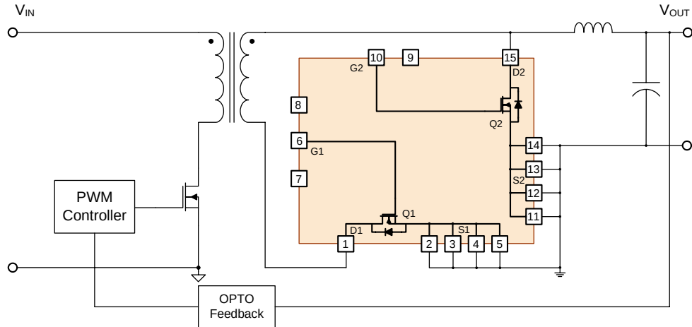
Figure 3. Application Circuit of Forward Converter with FD6M045N06
