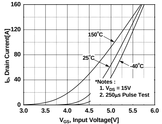
Figure 4. Transfer Characteristics
