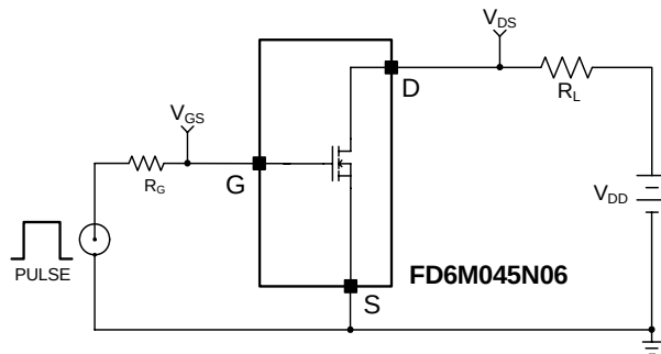
Figure 13. Switching Test Circuit
