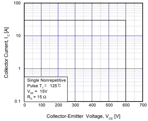
Fig 14. RBSOA Characteristics
