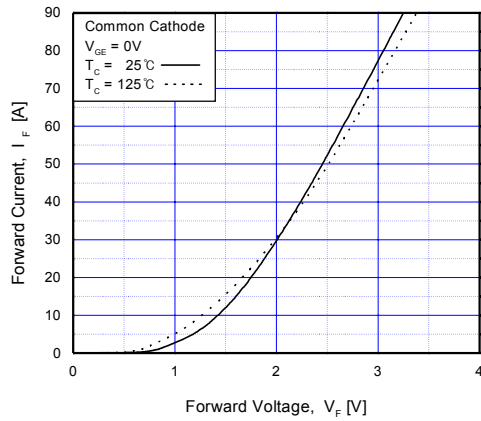
Fig 15. Forward Characteristics
