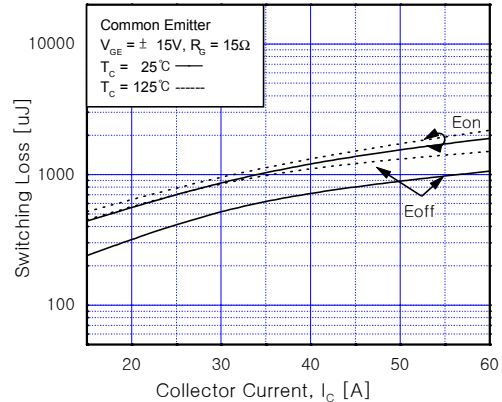
Fig 12. Switching Loss vs. Collector Current
