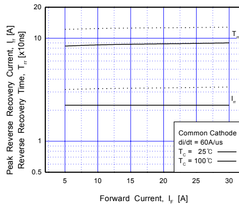
Fig 16. Reverse Recovery Characteristics
