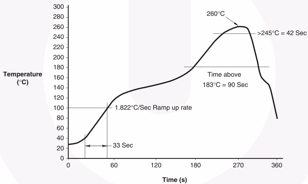
Reflow Profile
