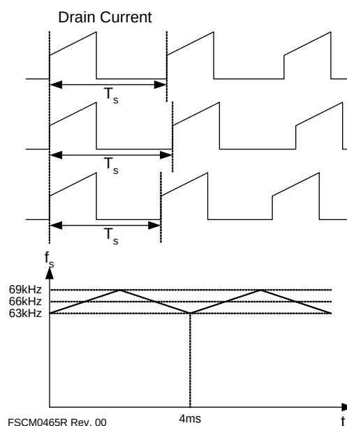
Figure 22. Frequency Modulation
