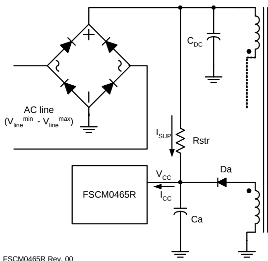
Figure 16. Startup Circuit
