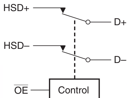
Figure 2. Analog Symbol
