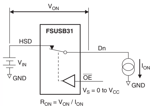
Figure 9. On Resistance
