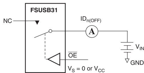
Figure 10. Off Leakage
