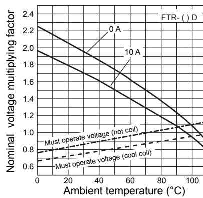
Operating range
