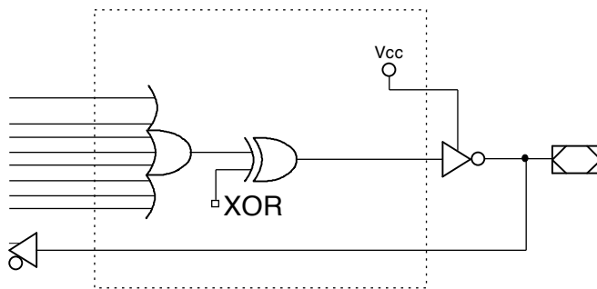
Combinatorial Output with Feedback Configuration for Simple Mode
