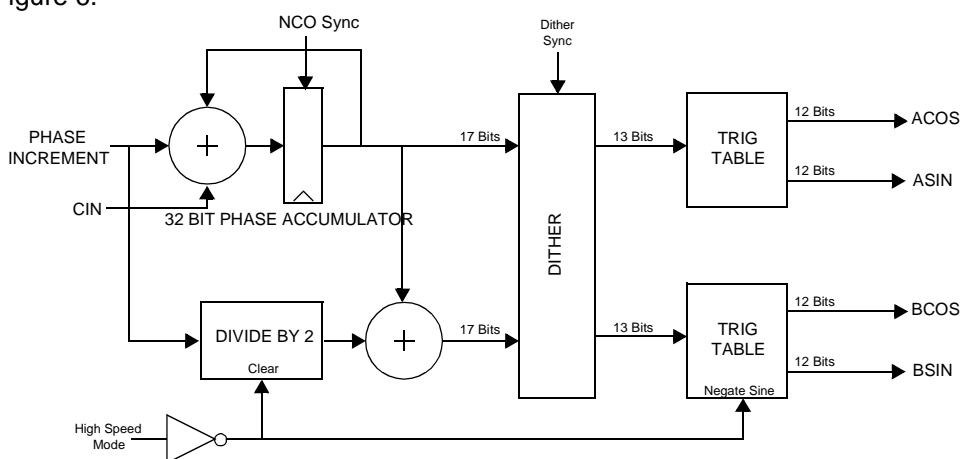
Figure 6. NCO CIRCUIT
