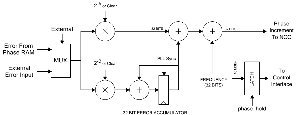
Figure 5. PLL CIRCUIT
