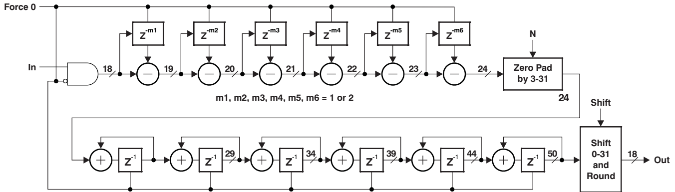
Figure 2-9. CIC Filter
