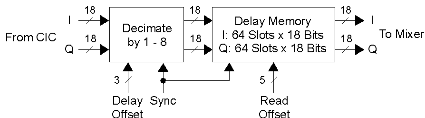
Figure 2-10. Delay Adjustment
