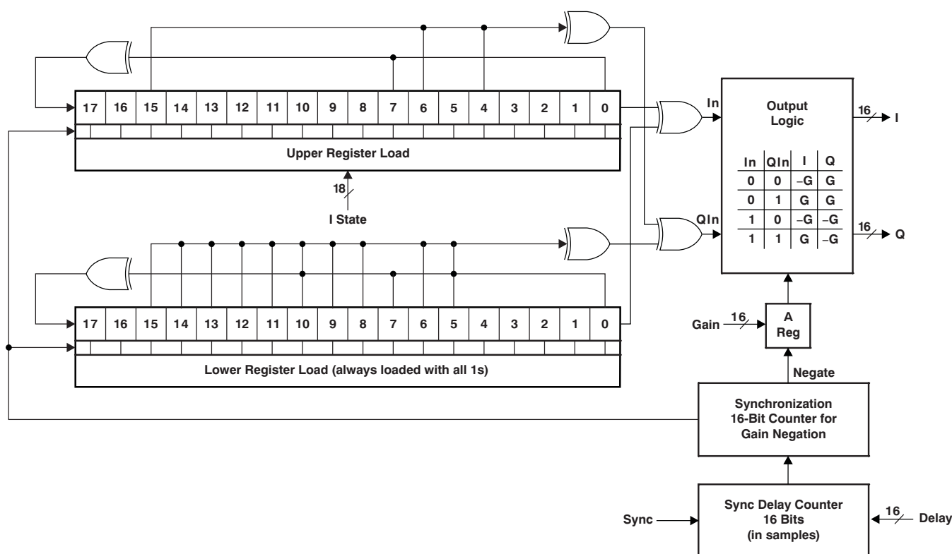
Figure 2-6. Pilot Code Insertion Logic
