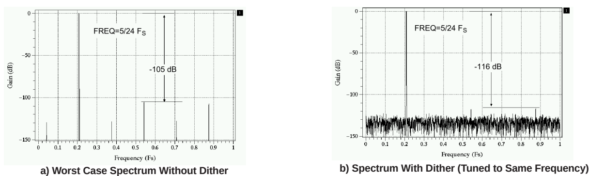
Figure 2-13. Example NCO Spurs With and Without Dithering
