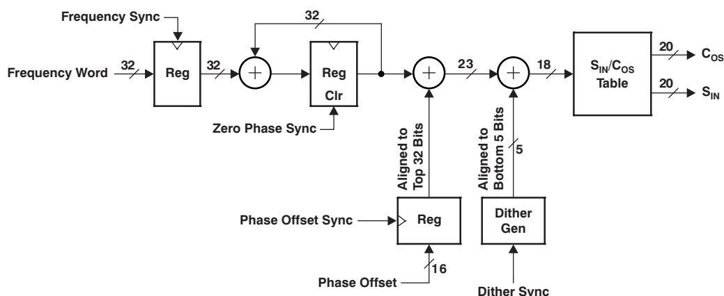
Figure 2-12. NCO
