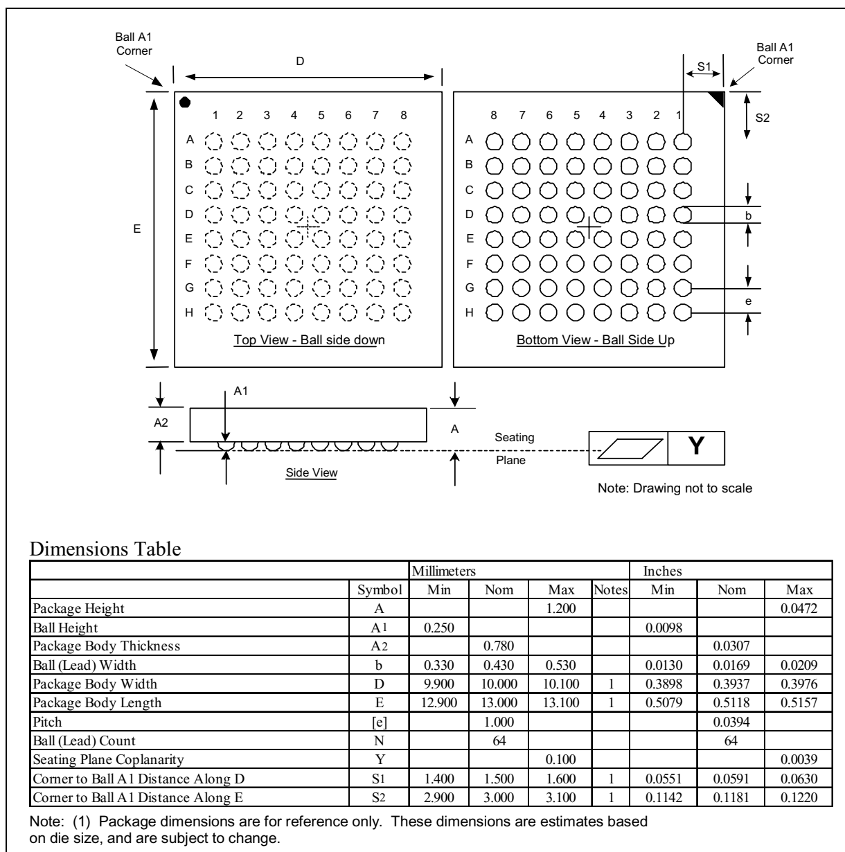
Figure 21. Easy BGA Package Drawing &amp; Dimension
