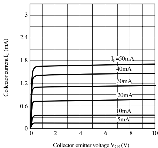
Fig.5 Collector Current vs. Collector-emitter Voltage
