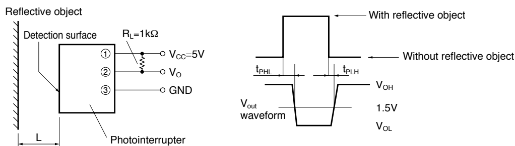
Fig.3 Test Circuit for Response Time
