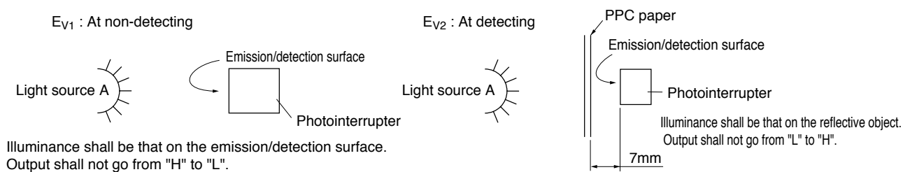
Fig.4 Test Condition for External Disturbing Light Illuminance
