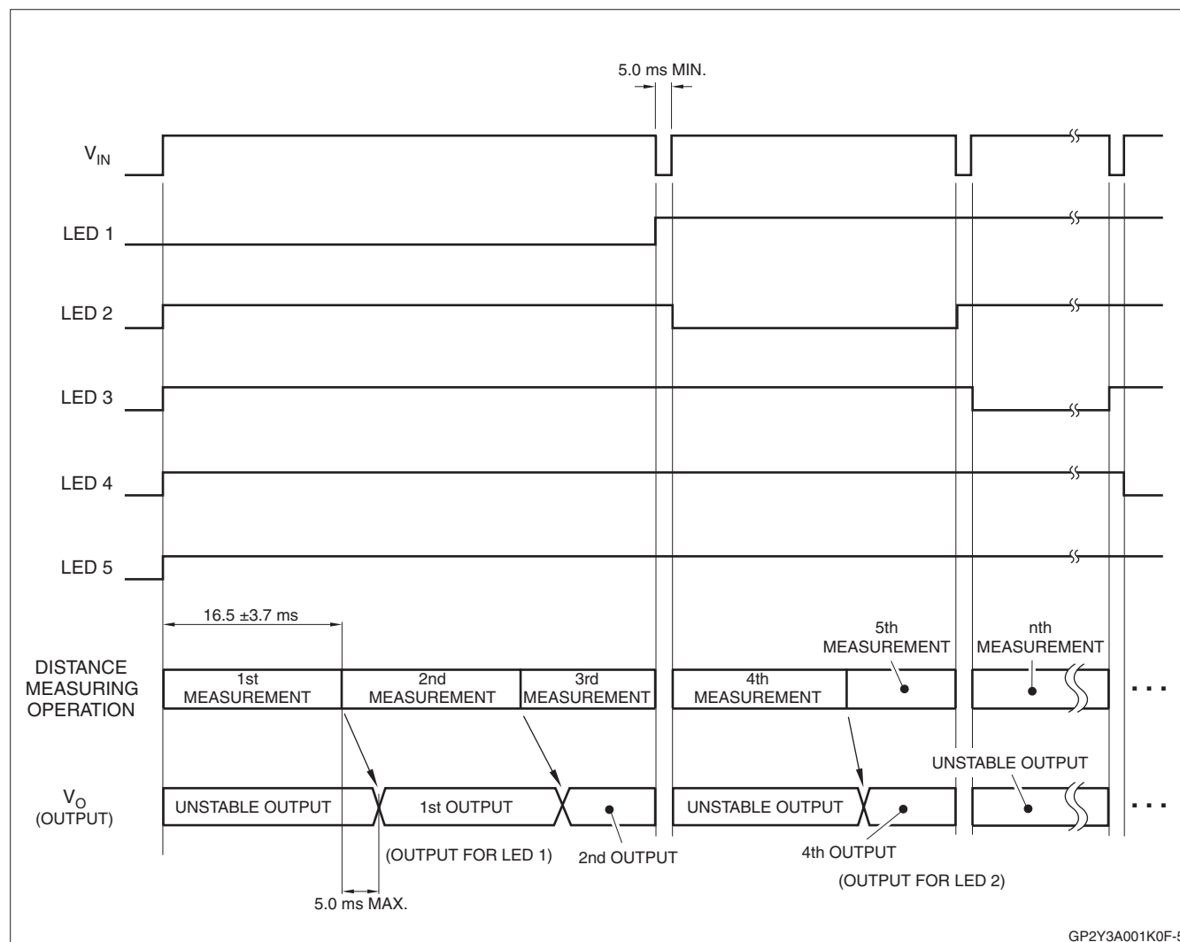
Figure 3. Timing Diagram
