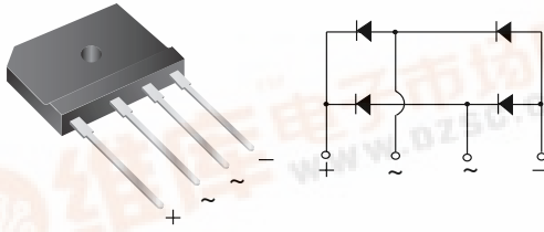
Case Style GSIB-5S
