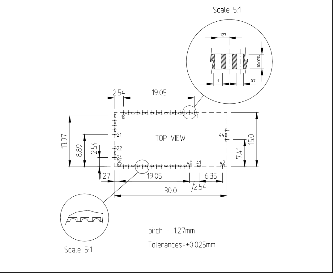
Figure 2. Mechanical dimensions
