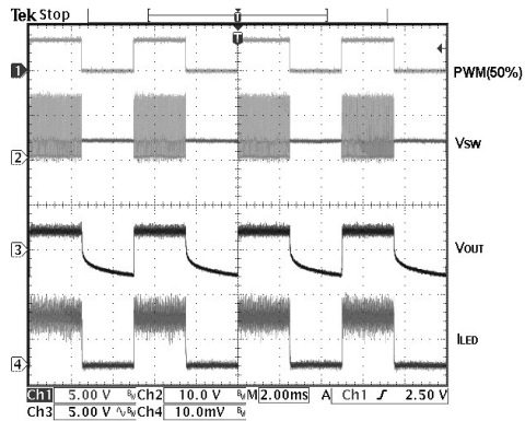
PWM Dimming
