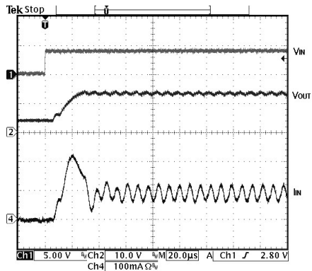
G5119 Inrush Current Waveform
