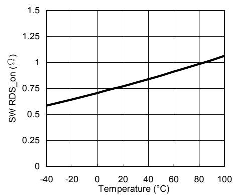
SW RDS on vs. Temperature
