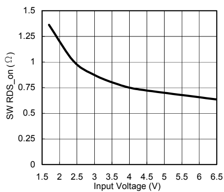
SW RDS on vs. Input Voltage
