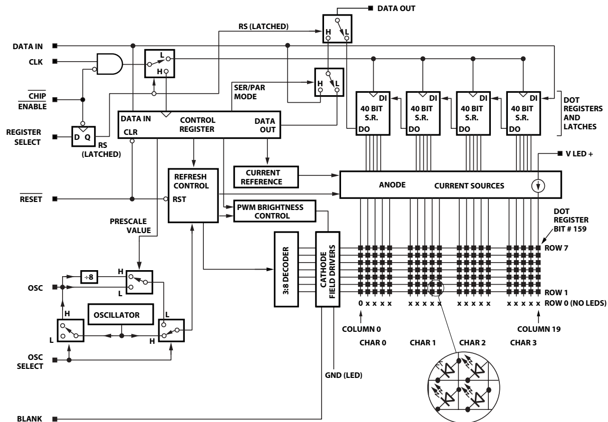
Figure 5. Block diagram
