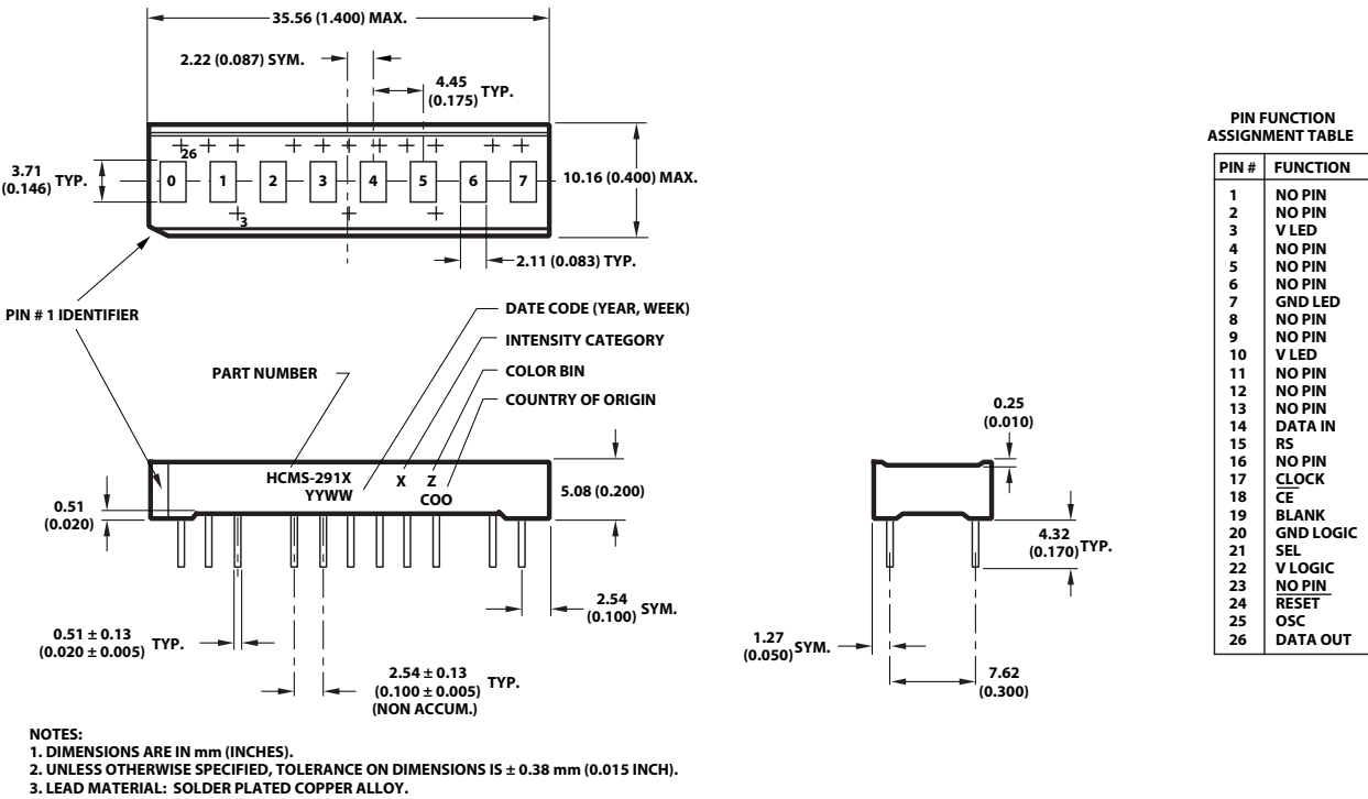
Figure 1. HCMS-2919 package dimension
