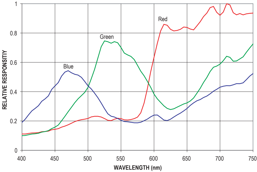
Figure 1. Spectral Responsivity
