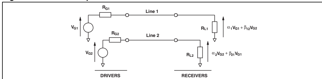
Figure 22. Crosstalk phenomena
