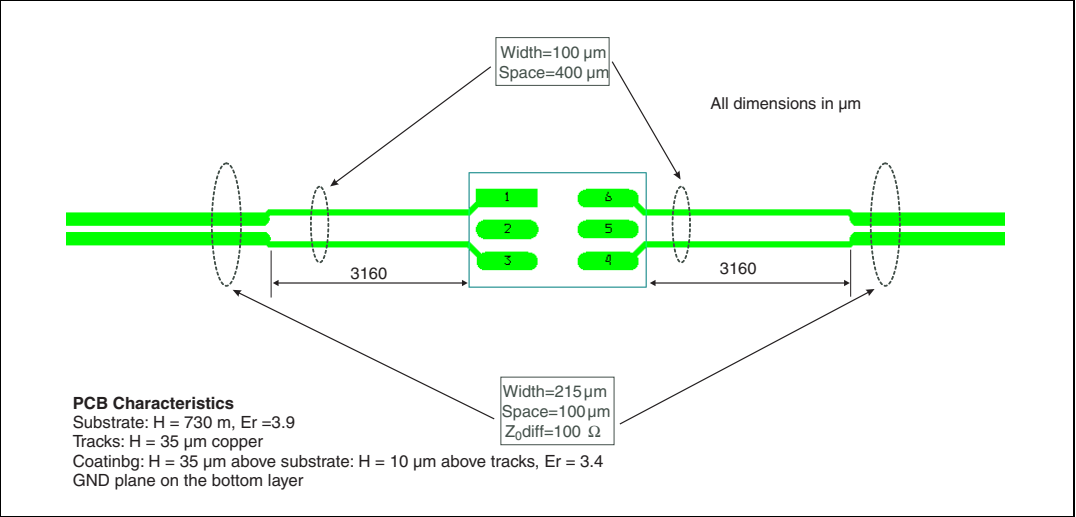
Figure 14. PCB layout example
