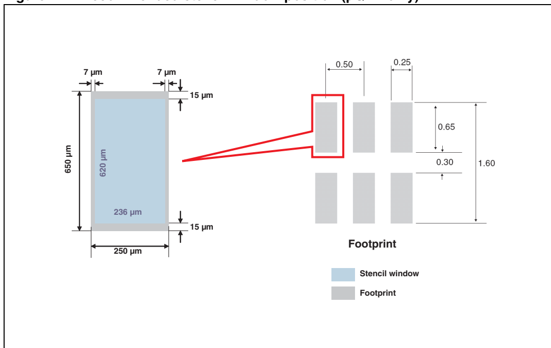
Figure 27. Recommended stencil window position ( \mu\text{QFN} only)
