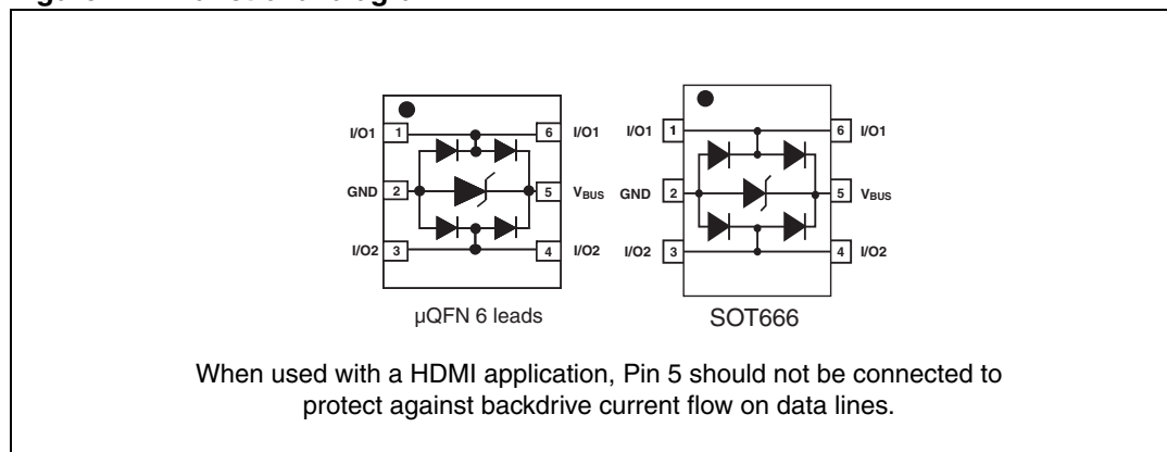
Figure 1. Functional diagram
