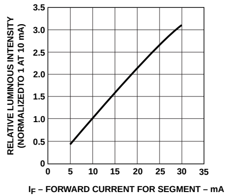
Figure 15. Relative luminous intensity vs. DC forward current.
