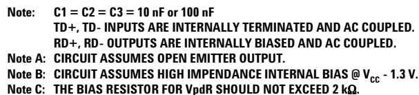
Figure 6. Recommended Interface Circuit
