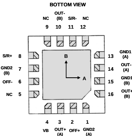
HMC1053 Pinout
