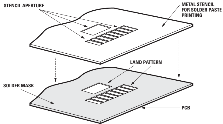
Figure 10. Stencil and PCBA.
