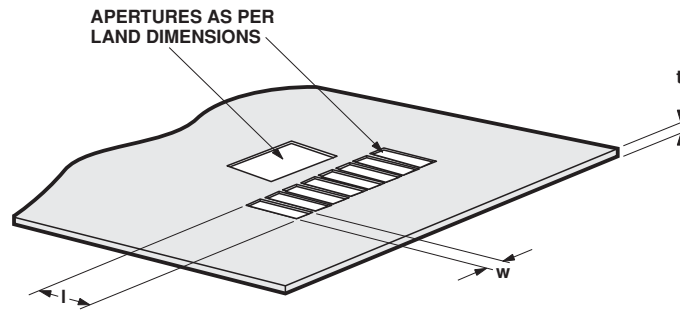
Figure 12. Solder stencil aperture.
