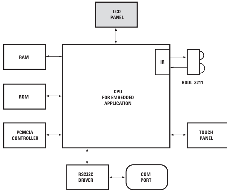
Figure 16. PDA platform.
