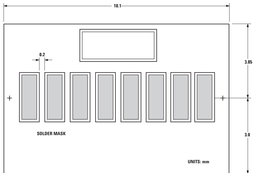
Figure 13. Adjacent land keepout and solder mask areas.
