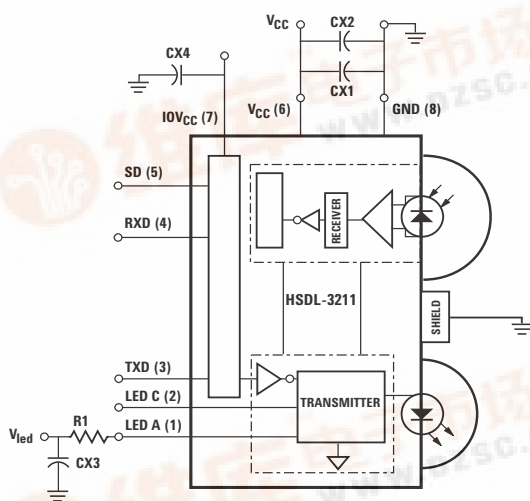
Figure 1. Functional block diagram of HSDL-3211.
