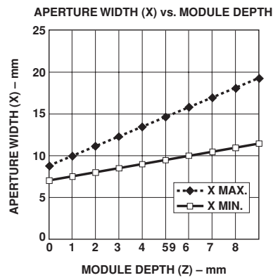
Figure 20. Aperture width (X) vs. module depth.
