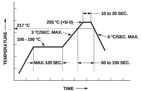
Figure 8. Recommended Pb-free reflow soldering profile.
