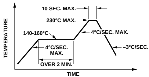
Figure 7. Recommended reflow soldering profile.
