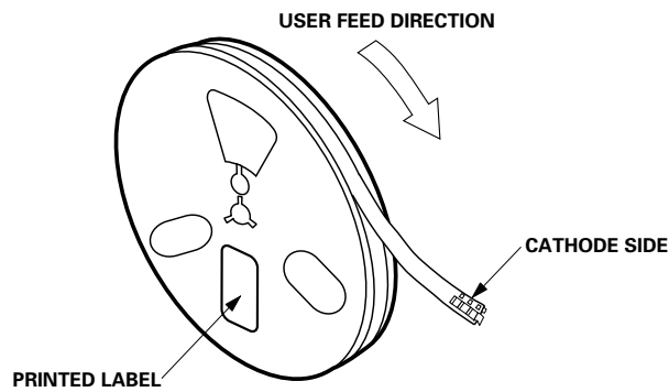
Figure 8. Reeling orientation.
